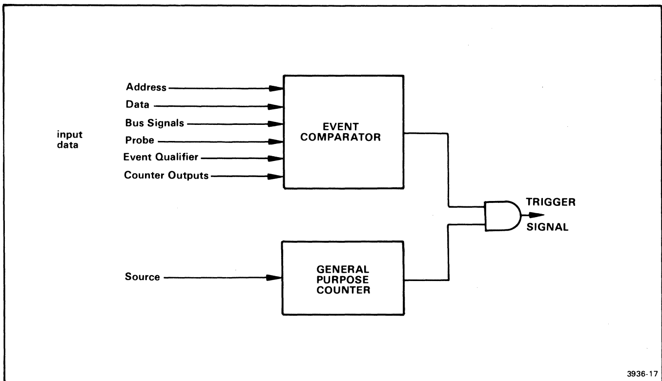
Fig. 5-6. Generating a trigger signal.
