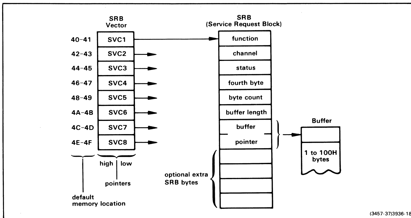
Fig. 6-1. SVC memory layout, Small Address Space (SAS) format.
