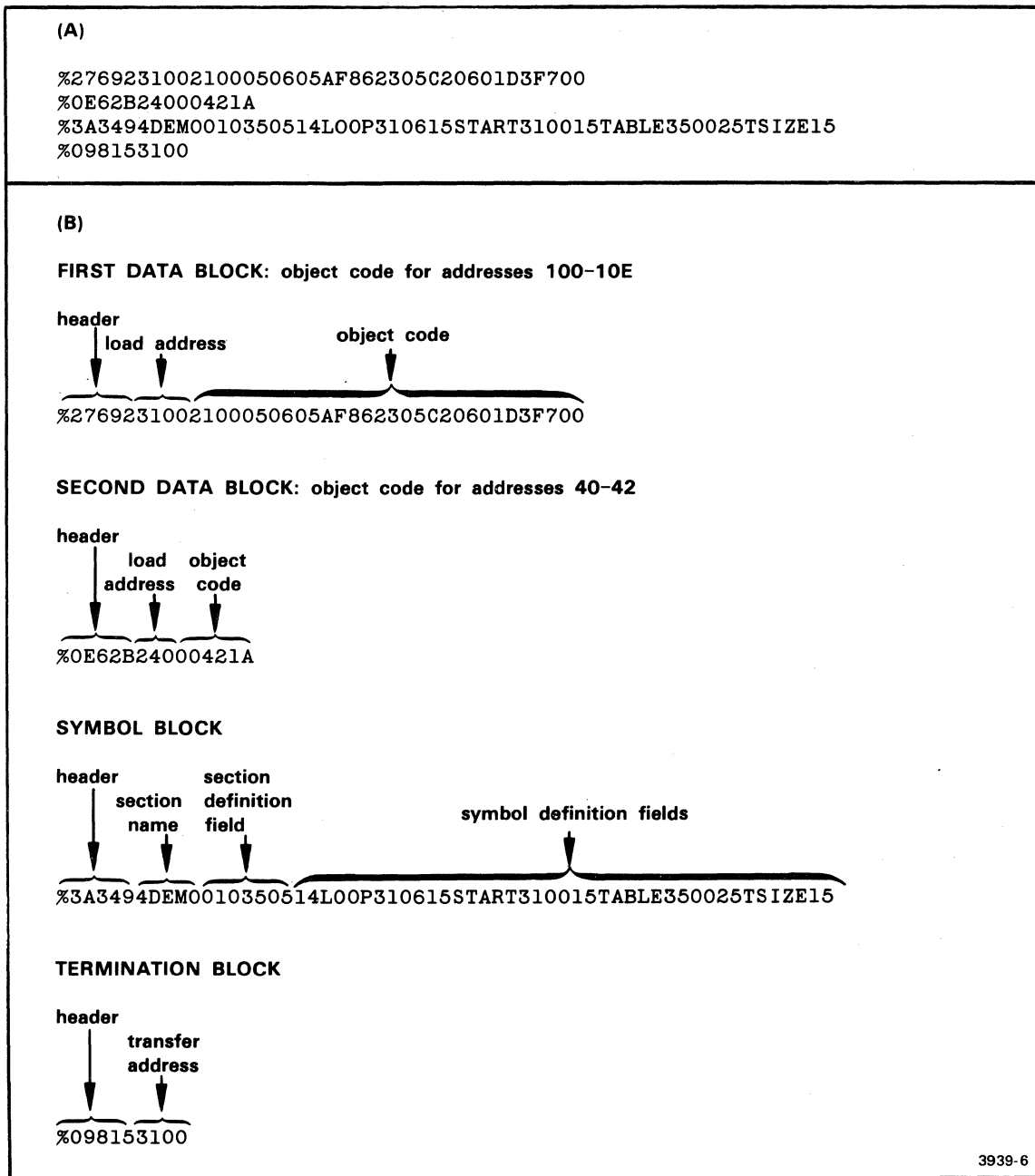
Fig. 1-4. Demonstration program: Extended Tekhex format.
