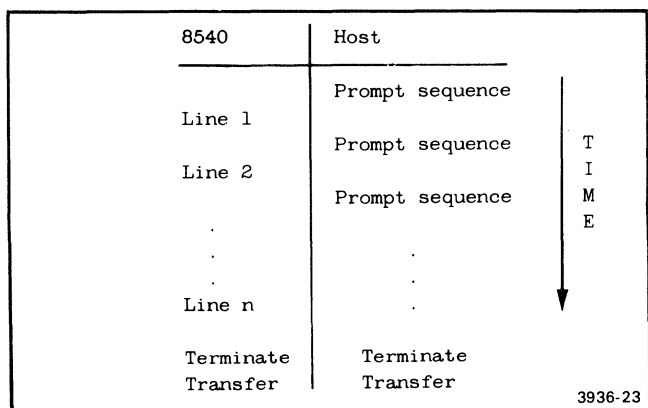
Fig. 4-2. Protocol for unformatted ASCII uploads.
