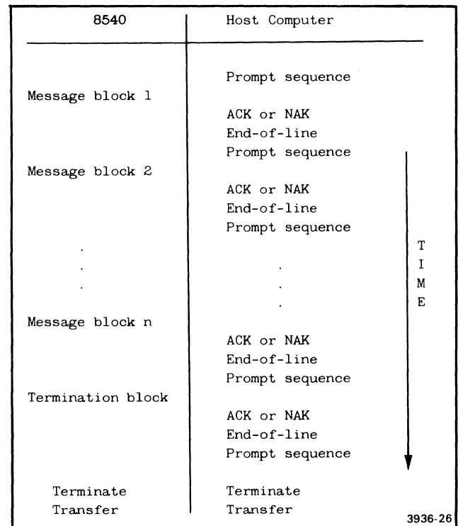
Fig. 4-5. Protocol for formatted uploads.
