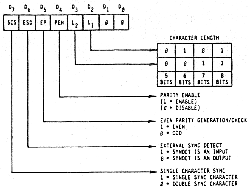
(a) SYNCHRONOUS MODE
