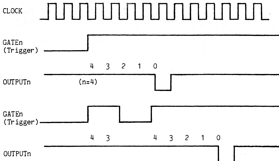
Figure 5-12 MODE 5 TIMING DIAGRAM
