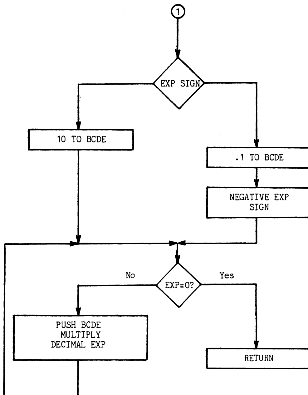
Figure 6 (cont'd) ASCII TO FLOATING POINT ROUTINE
