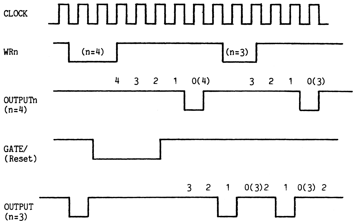
Figure 5-9 MODE 2 TIMING DIAGRAM
