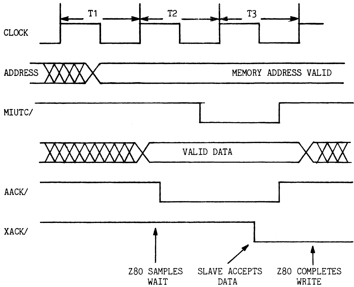
Figure 3-3 Z80 WRITE OPERATION
