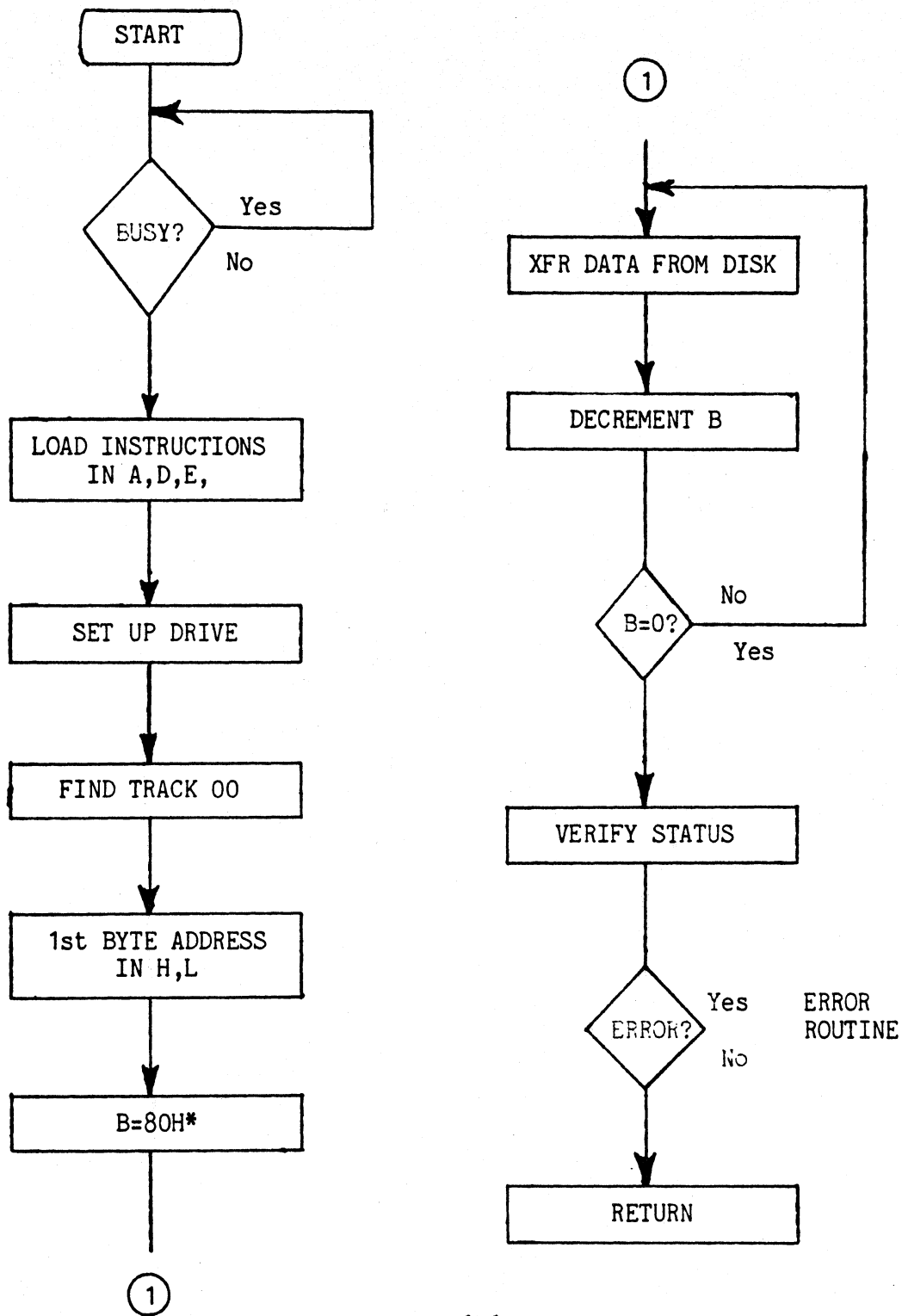
Figure 6-6 SECTOR READ ROUTINE
