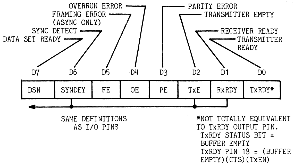
Figure 5-4 STATUS WORD FORMAT
