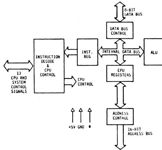
(b) BLOCK DIAGRAM
