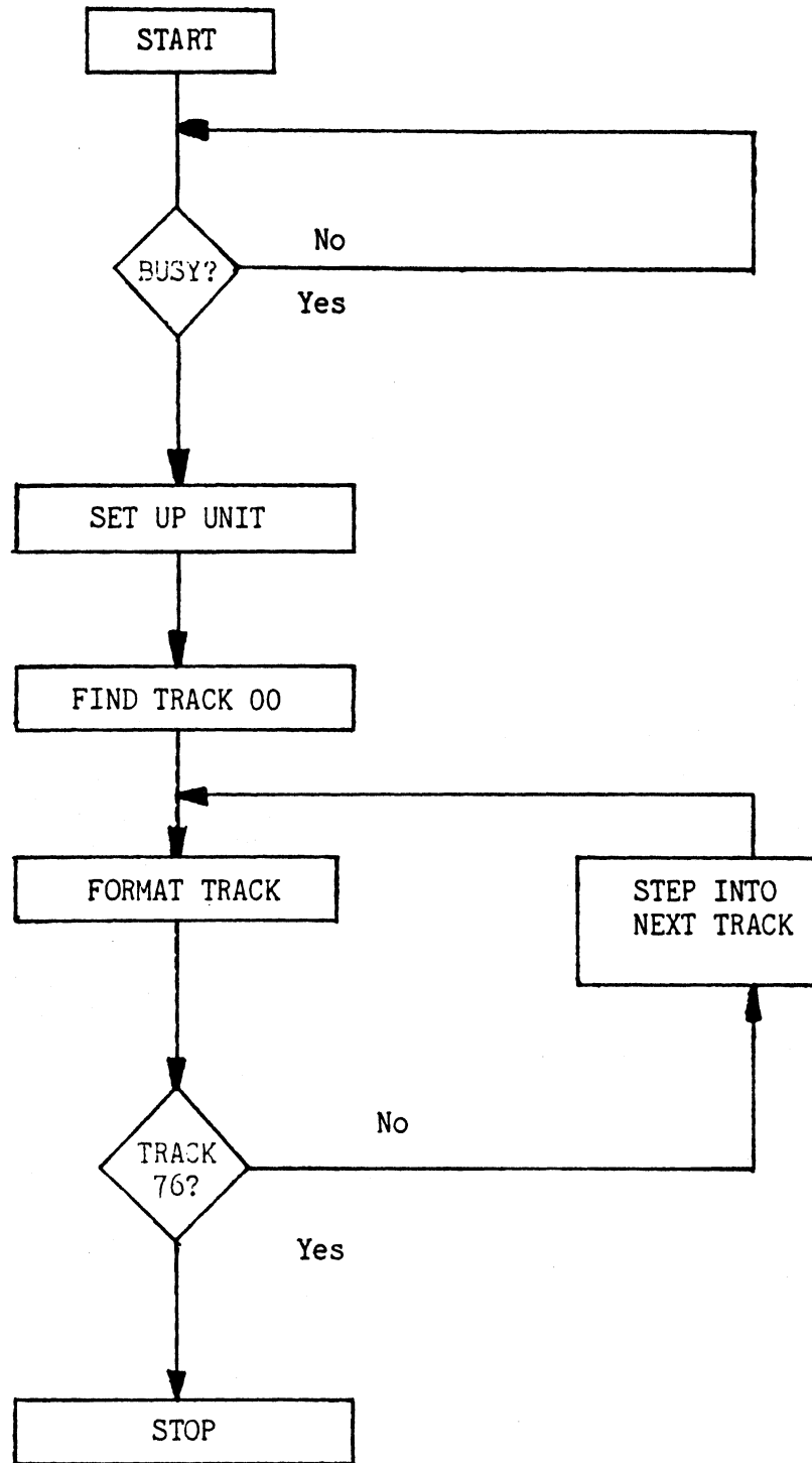
Figure 6-10 DISK INITIALIZATION ROUTINE
