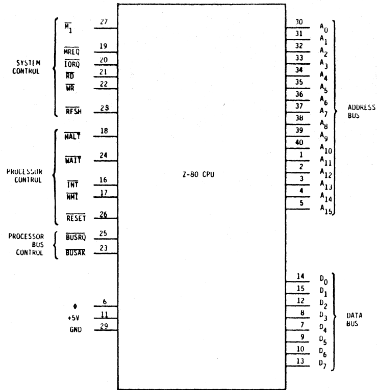
(a) PIN CONFIGURATION
