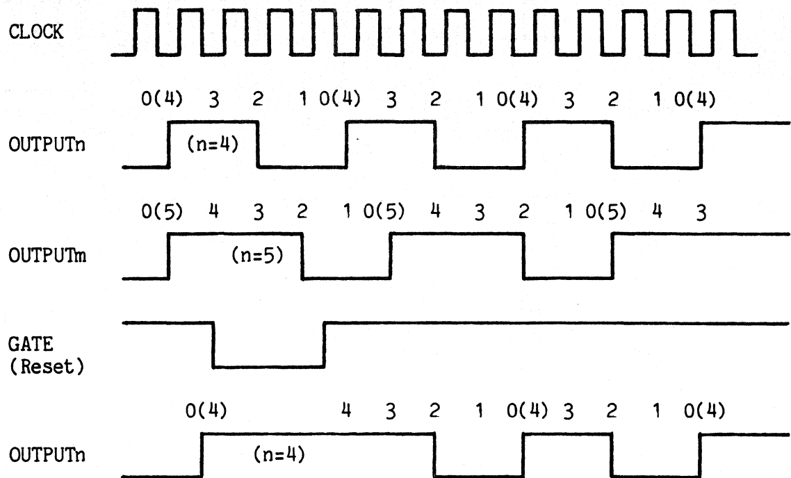
Figure 5-10 MODE 3 TIMING DIAGRAM
