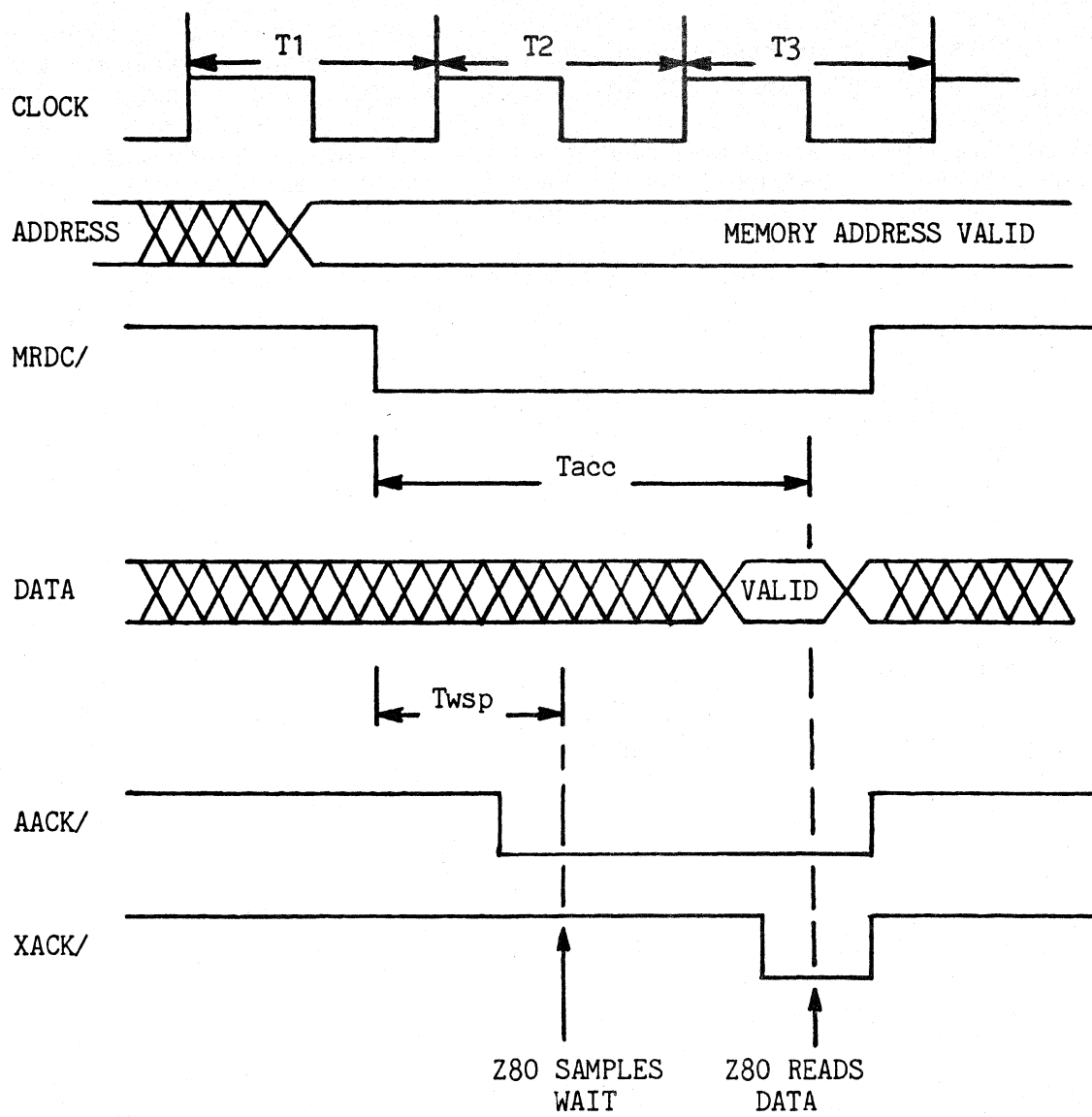
Figure 3-2 Z80 READ OPERATION
