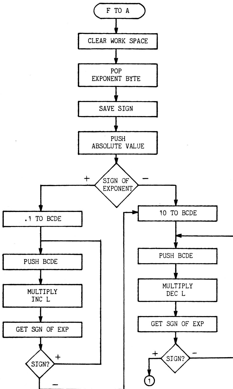
Figure 5 FLOATING POINT TO ASCII CONVERSION ROUTINE
