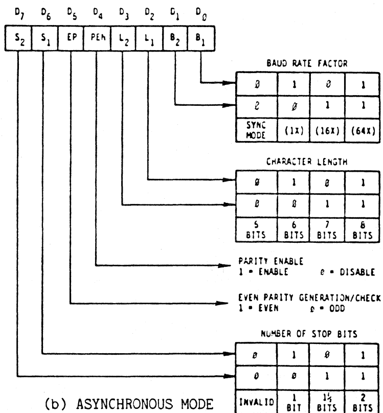
Figure 5-2 MODE INSTRUCTION CONTROL WORD FORMAT
