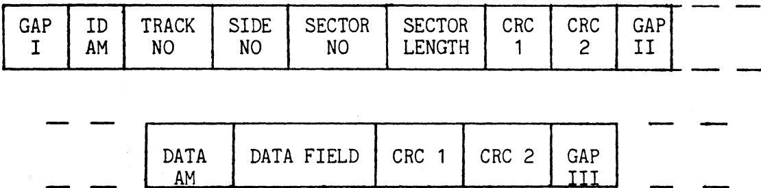
Figure 6-3 DISK SECTOR FORMAT
