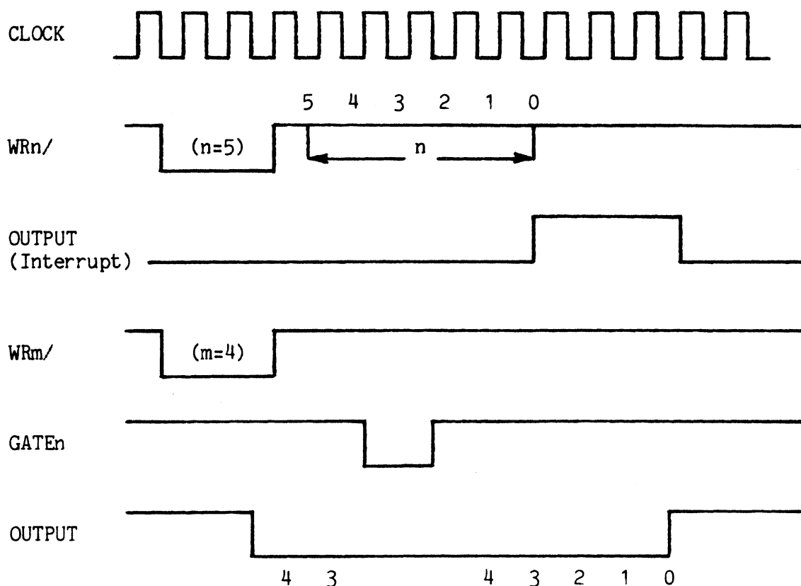
Figure 5-7 MODE 0 TIMING DIAGRAM
