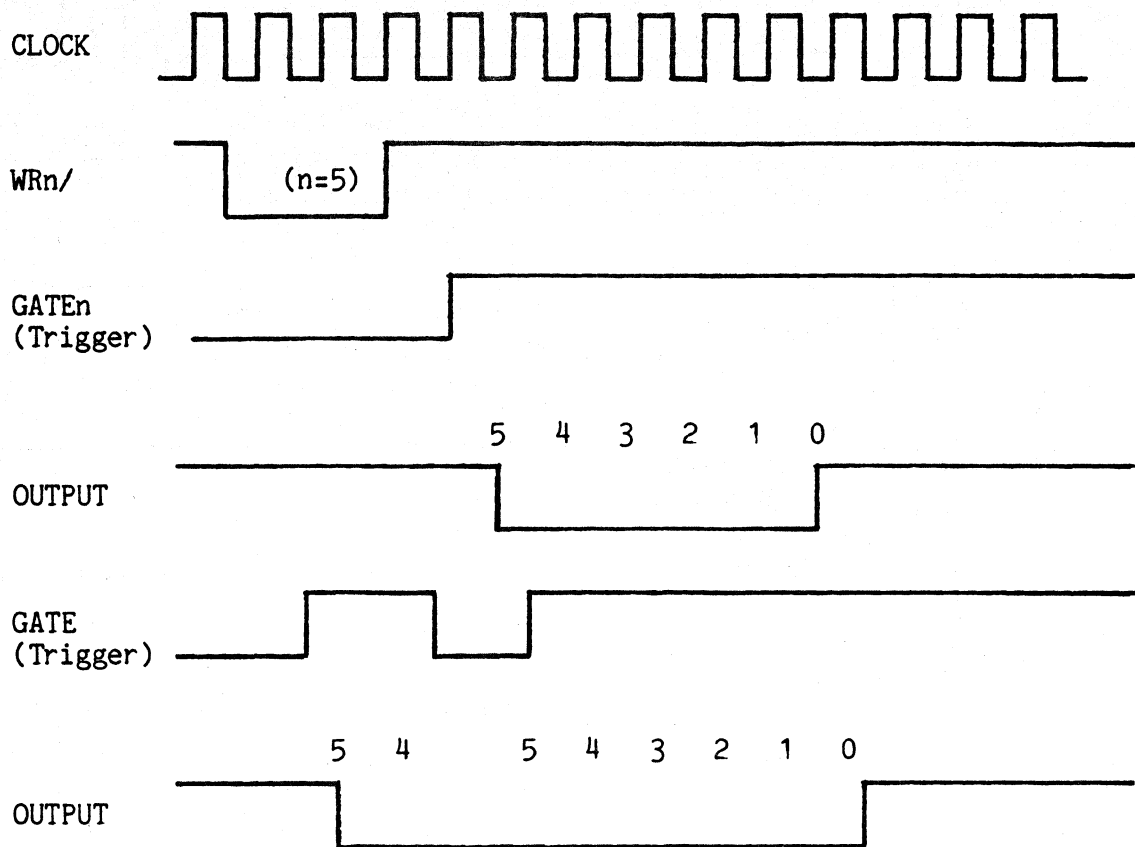
Figure 5-8 MODE 1 TIMING DIAGRAM
