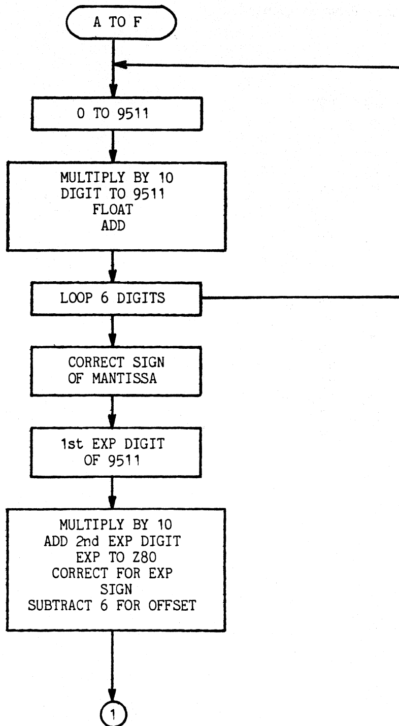
Figure 6 ASCII TO FLOATING POINT CONVERSION ROUTINE
