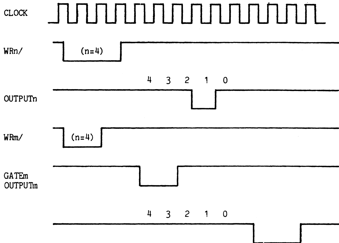
Figure 5-11 MODE 4 TIMING DIAGRAM
