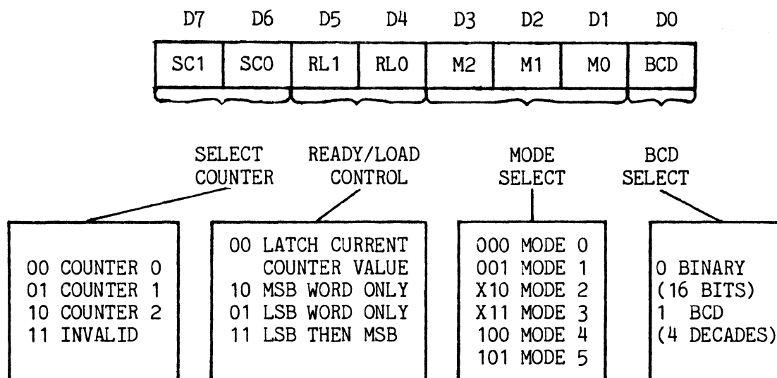
Figure 5-6 8253 INTERVAL TIMER CONTROL WORD FORMAT
