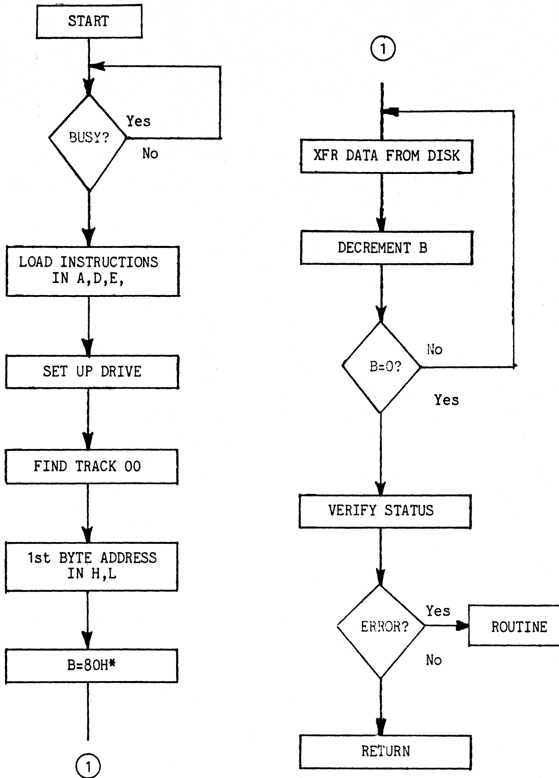
Figure 6-7 SECTOR WRITE ROUTINE
