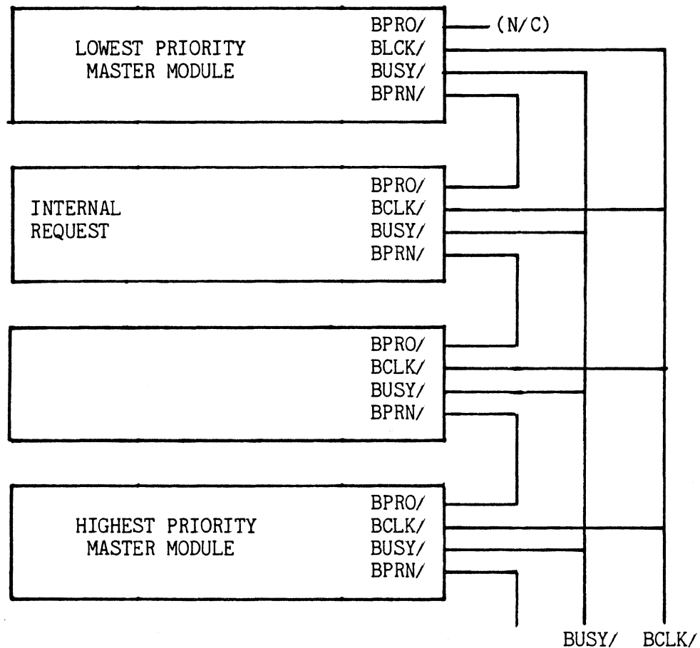
Figure 3-1 SERIAL-BUS CONTENTION CONFIGURATION
