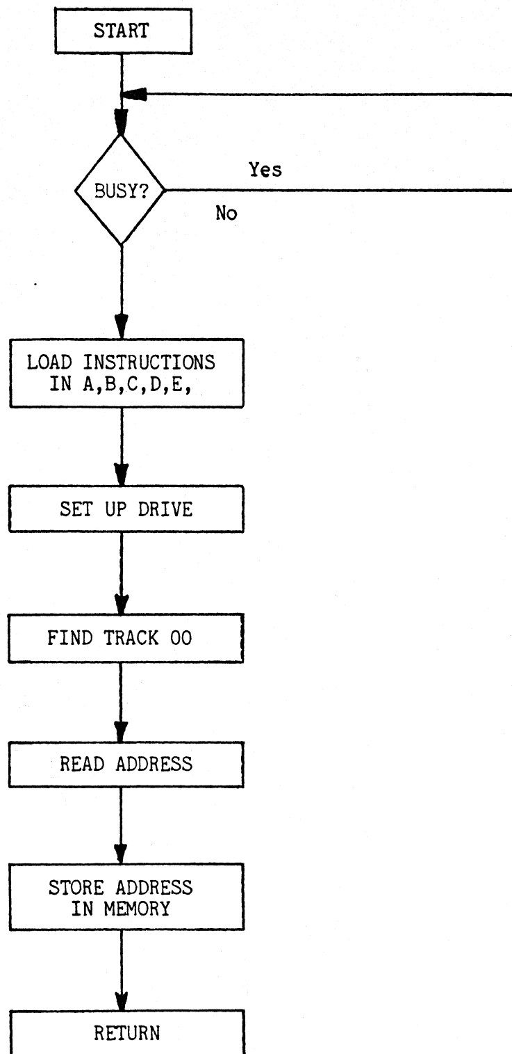
Figure 6-8 READ ADDRESS ROUTINE
