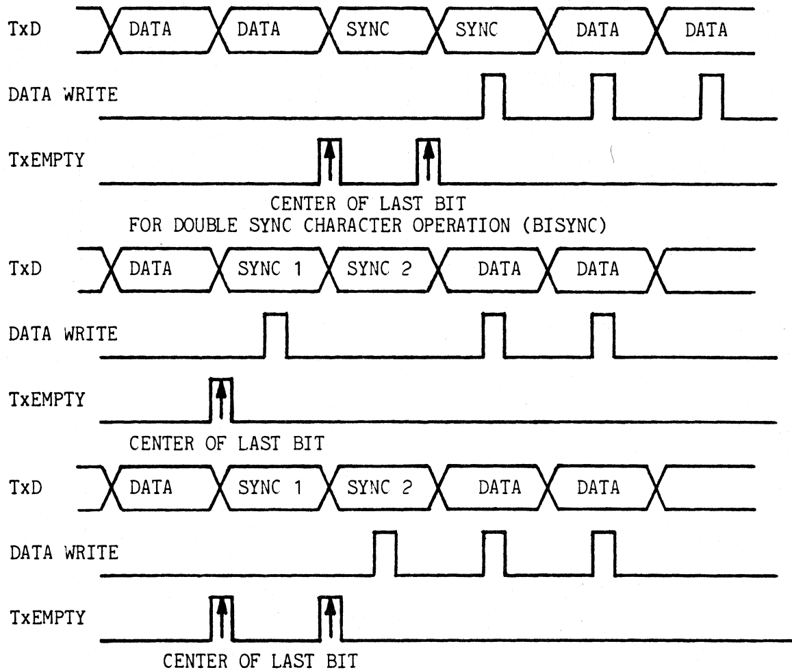
Figure 5-5 SYNC CHARACTER TRANSMISSION
