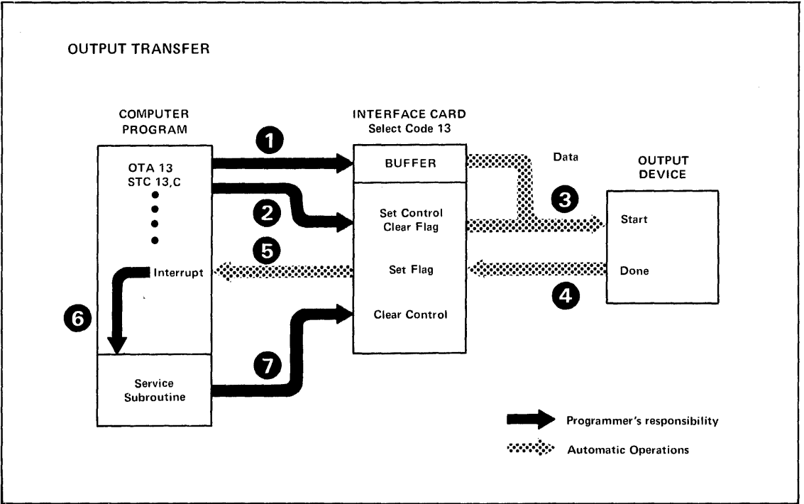
Figure 4.5. Input/Output Transfers (Part 2)
