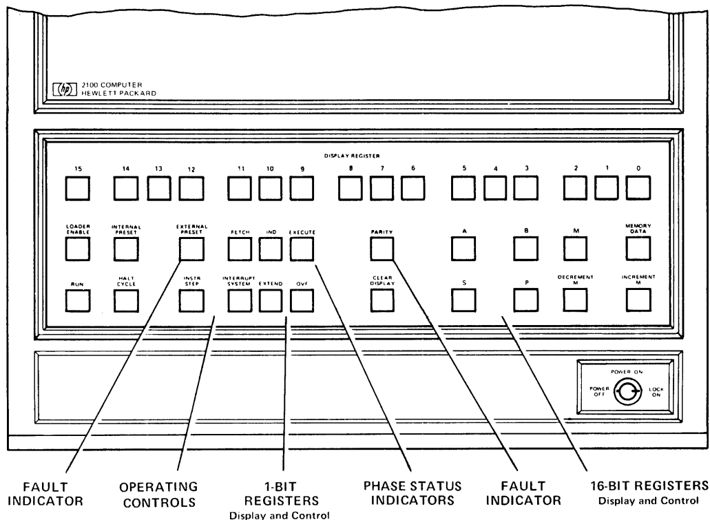
Figure 5.1. Operator Panel Controls and Indicators (Part 1)
