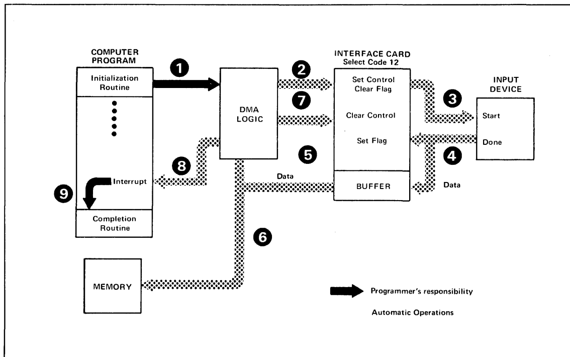
Figure 4.6. DMA Transfers
