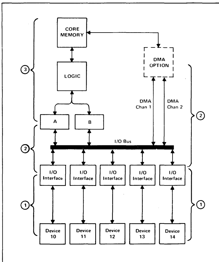
Figure 4.1. Input/Output System
