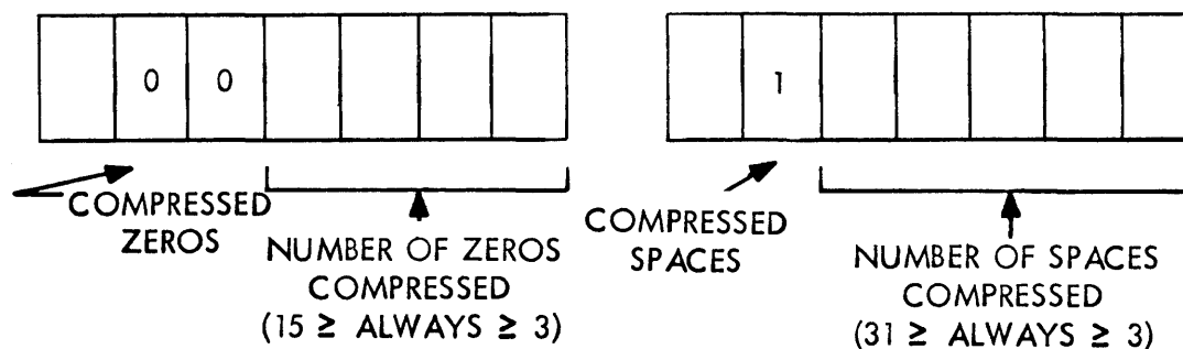
Figure 3-11. Compression Codes
