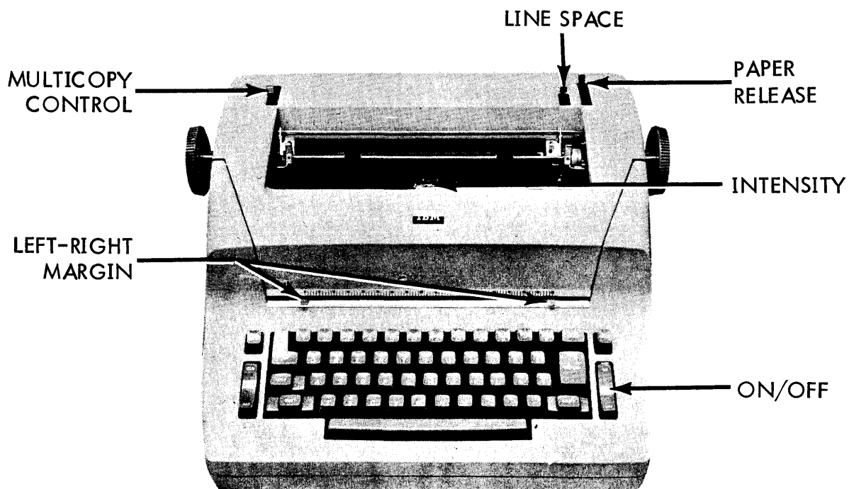
Figure 2-7. Typewriter Controls
