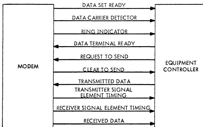
Figure 3-1. Interface Signals
