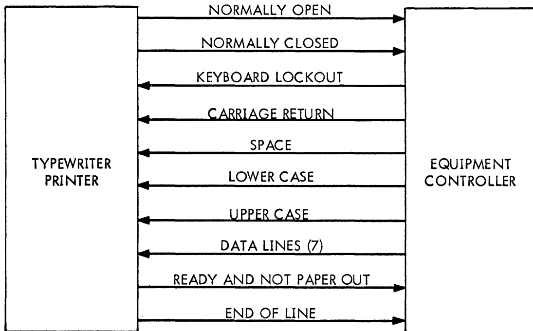
Figure 3-5. Typewriter Signals
