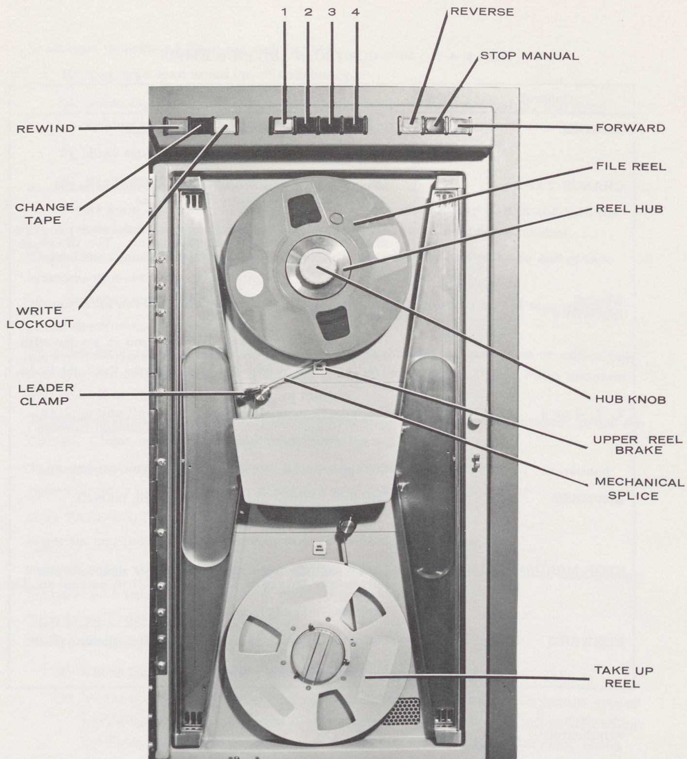
Figure 4-9. 1607 Tape Unit
