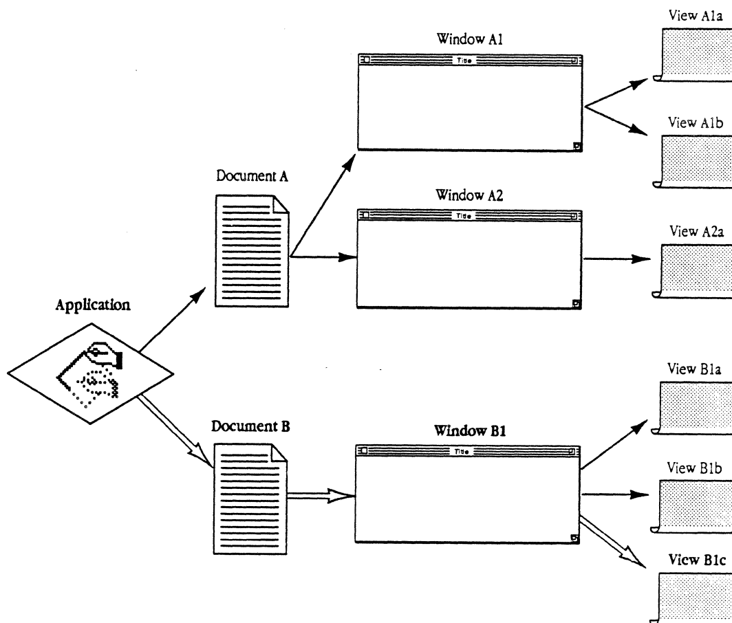
Figure 5-6 The command web
