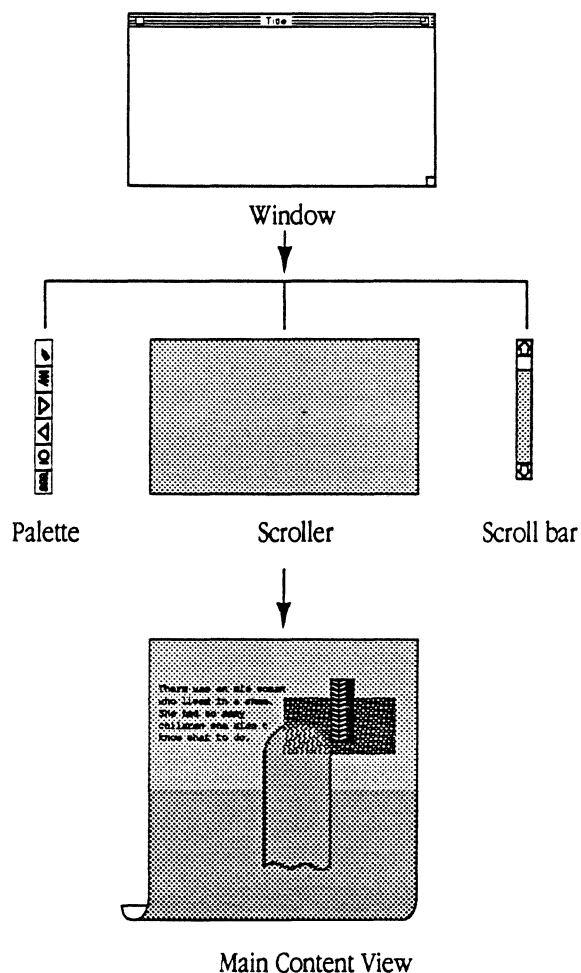
Figure 4-5 View tree for window in Figure 4-3
