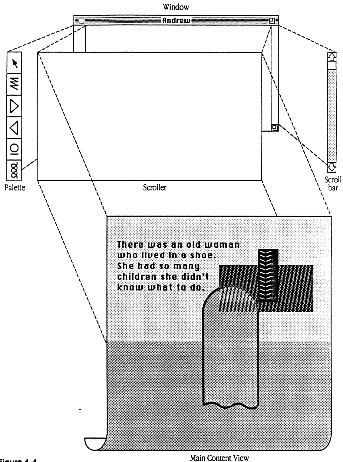
Figure 4-4 Blown-up version of window in Figure 4-3
