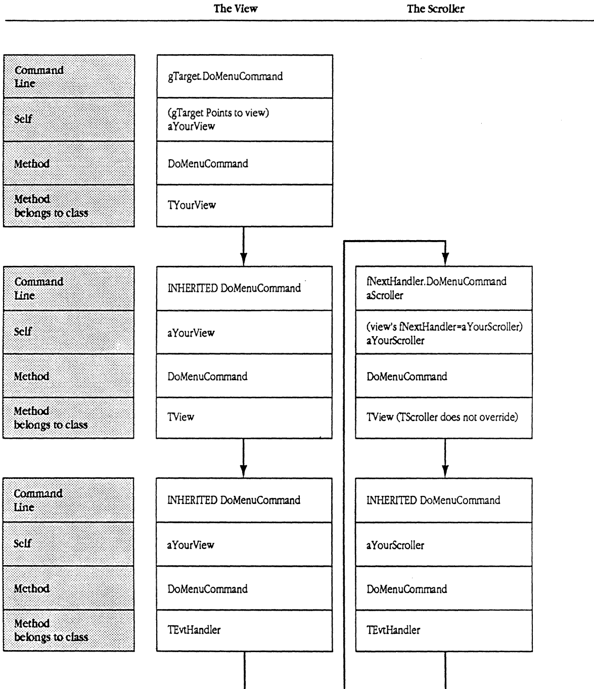
Figure 5-8 Example: The command chain when the user chooses Quit
