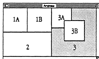
Figure 5-9 The view tree
