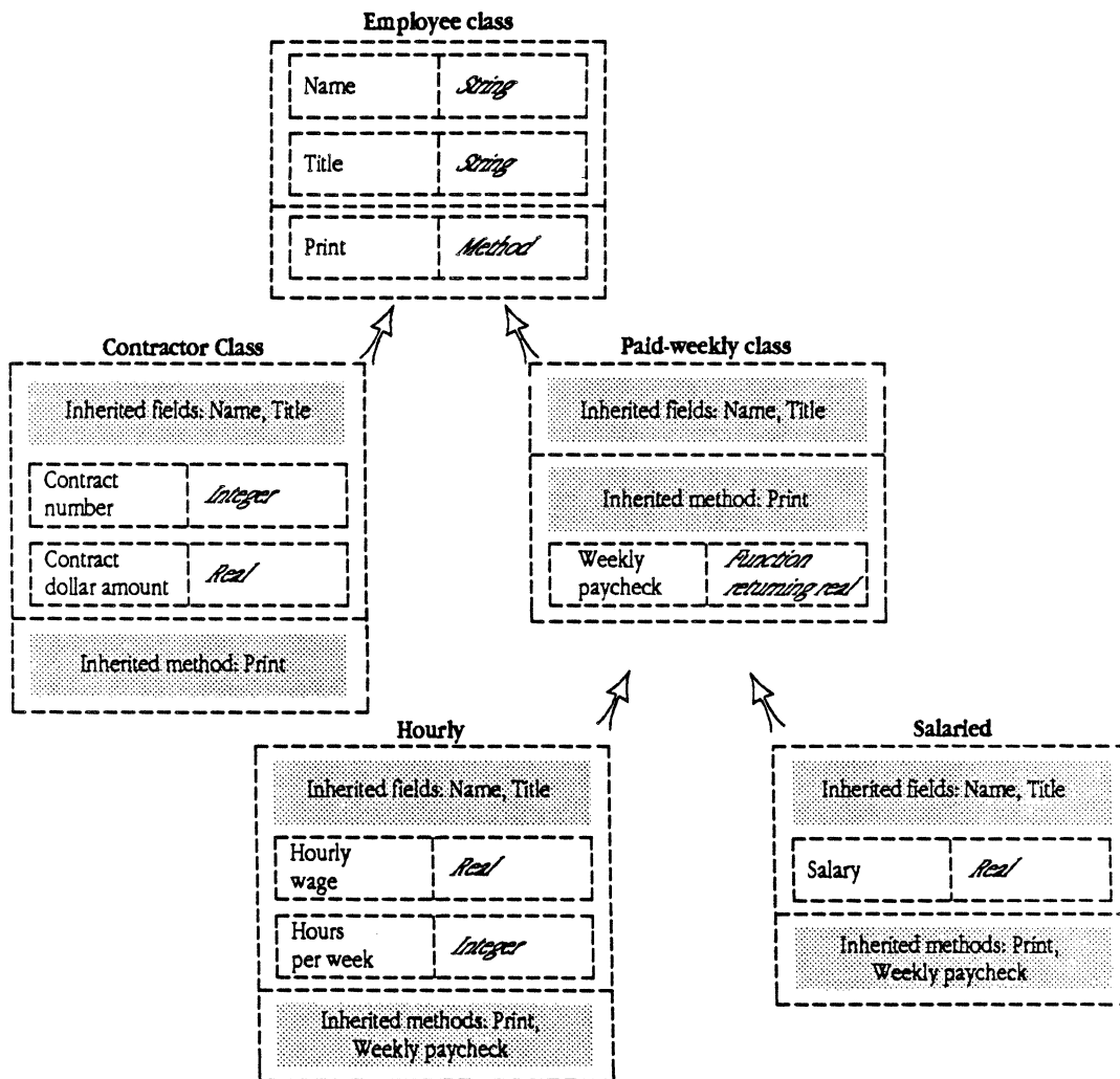
Figure 2-18 Multiple levels of inheritance
