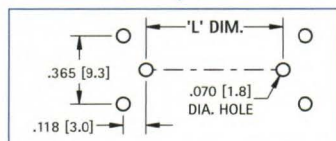
Mounting Detail
