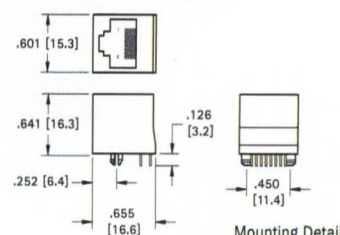
Mounting Detail
