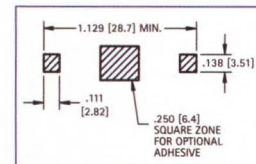
Pad Layout
