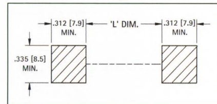
Pad Layout
