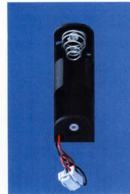
6" Wire Leads with 3 Pin Locking PC Connector (CN)
