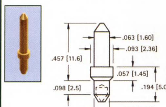
.063 (1.6) PIN - SWAGE MOUNT
