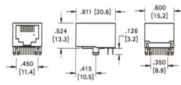
Mounting Detail
