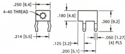
Mounting Detail
