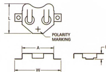
FIG. 2 - Low Profile
