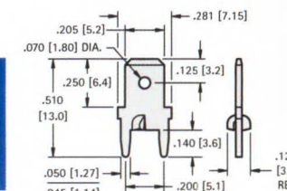
.205 (5.2) TAB
