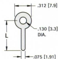
MATERIAL: .020 (.51) Brass, Tin Plate
