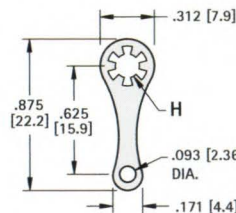
MATERIAL: .018 (.46) Brass, Tin Plate
