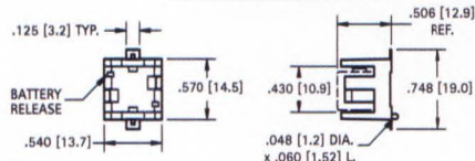
SURFACE MOUNT
