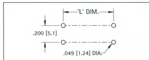
Mounting Detail
