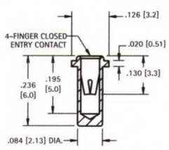
.032 (.81) - .046 (1.17) PIN - SOLDER MOUNT
