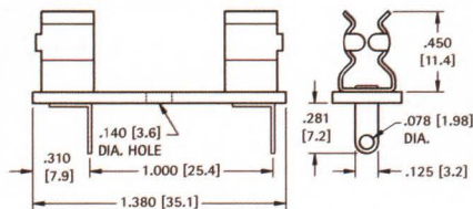
Mounting Detail
