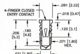
.032 (.81) - .046 (1.17) PIN - PRESS-FIT
