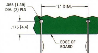
Fig. 5 Off-Board Mount
