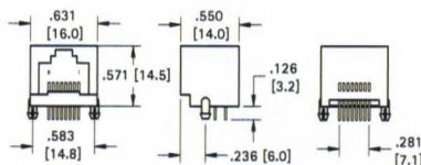
Mounting Detail
