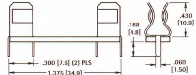
Mounting Detail
