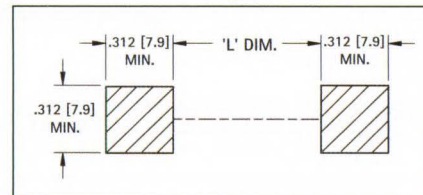
Pad Layout
