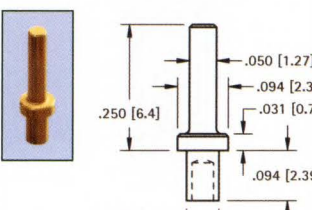
.050 (1.3) PIN - SWAGE MOUNT
