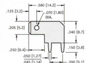
.205 (5.2) TAB
