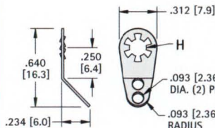
MATERIAL: .018 (.46) Brass, Tin Plate
