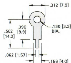
MATERIAL: .016 (.41) Brass, Tin Plate CAT. NO. 680
