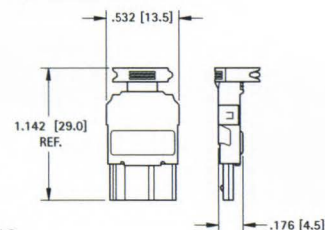
CABLE PLUG
