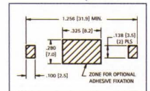
Pad Layout
