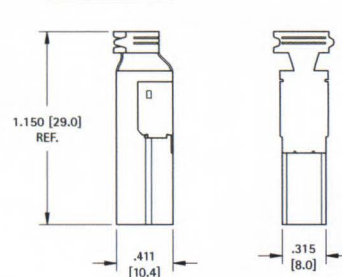
CABLE PLUG
