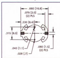
Pad Layout
