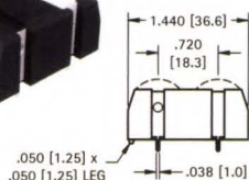
Mounting Detail
