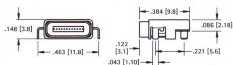
Mounting Detail
