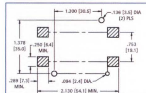
Pad Layout
