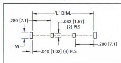
Mounting Detail
