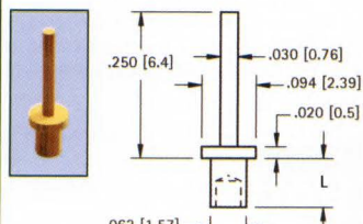
.030 (.76) PIN - SWAGE MOUNT
