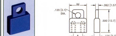
INSULATED SHORTING JACK
