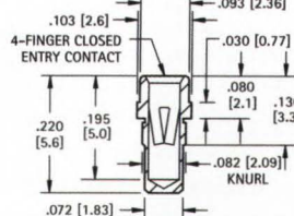
.032 (.81) - .046 (1.17) PIN - PRESS-FIT
