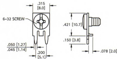
Mounting Detail
