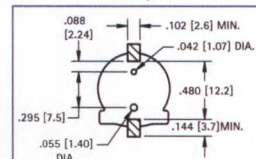
Pad Layout
