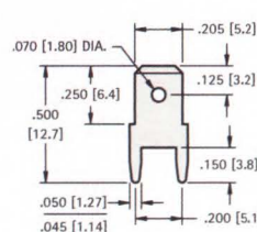
.205 (5.2) TAB
