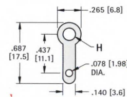
MATERIAL: .020 (.51) Brass, Tin Plate
