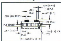
Mounting Detail
