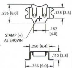
Mounting Detail
