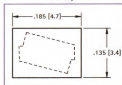
Pad Layout
