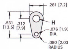
MATERIAL: .015 (.38) Brass, Tin Plate
