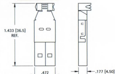
CABLE PLUG
