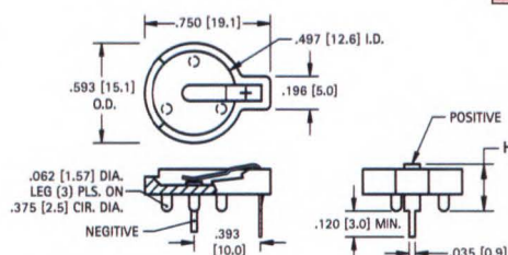
Mounting Detail
