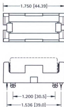
Mounting Detail
