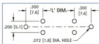
Mounting Detail
