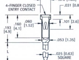
IC SOCKET CONTACTS FOR .015 (.38) - .025 (.64) LEADS - PRESS-FIT
