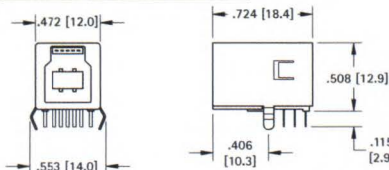
Mounting Detail
