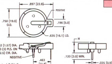
Mounting Detail
