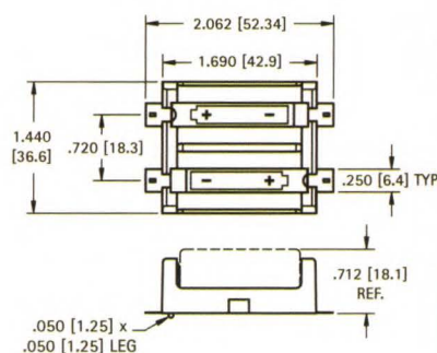
Mounting Detail
