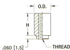
THREADED STANDOFFS
